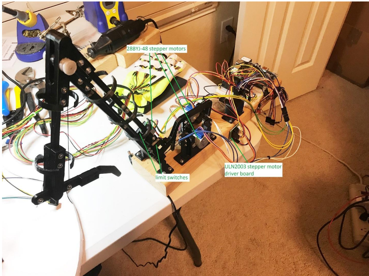
Leg test rig
