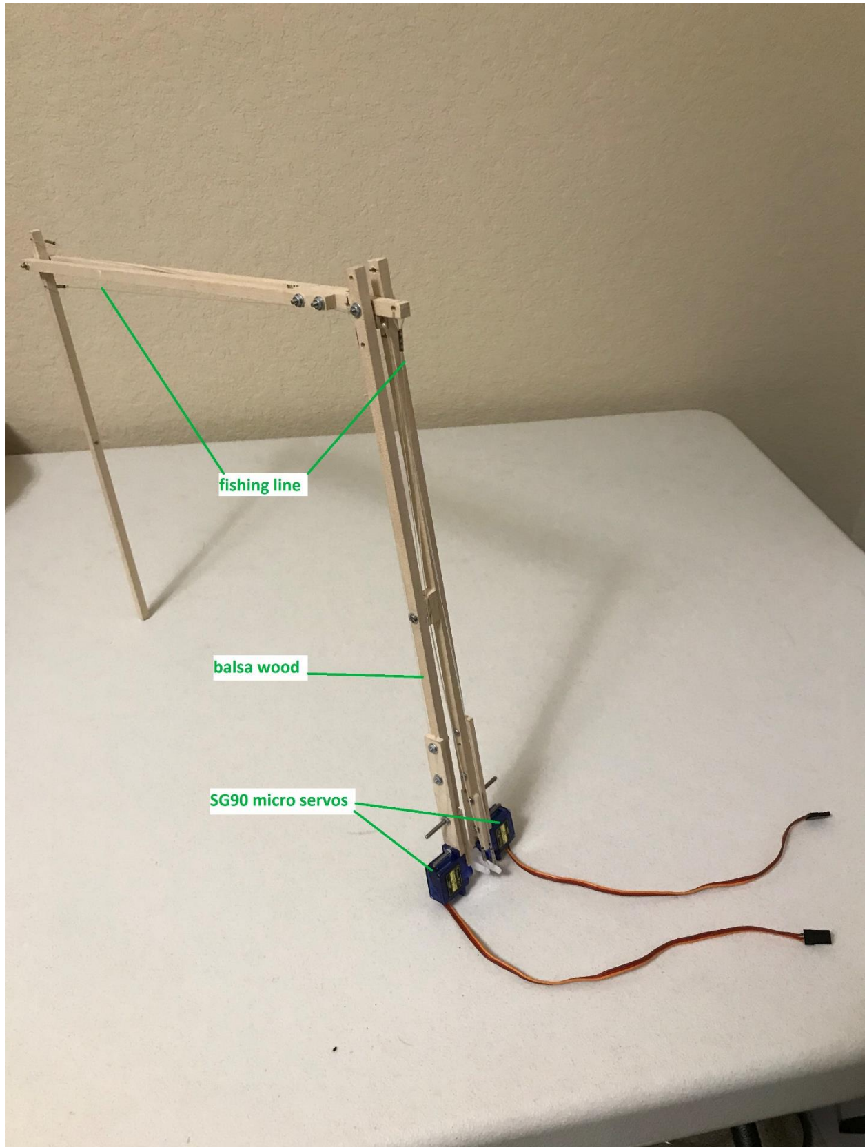
Leg: first prototype
