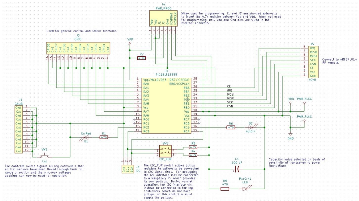
Main control circuit
