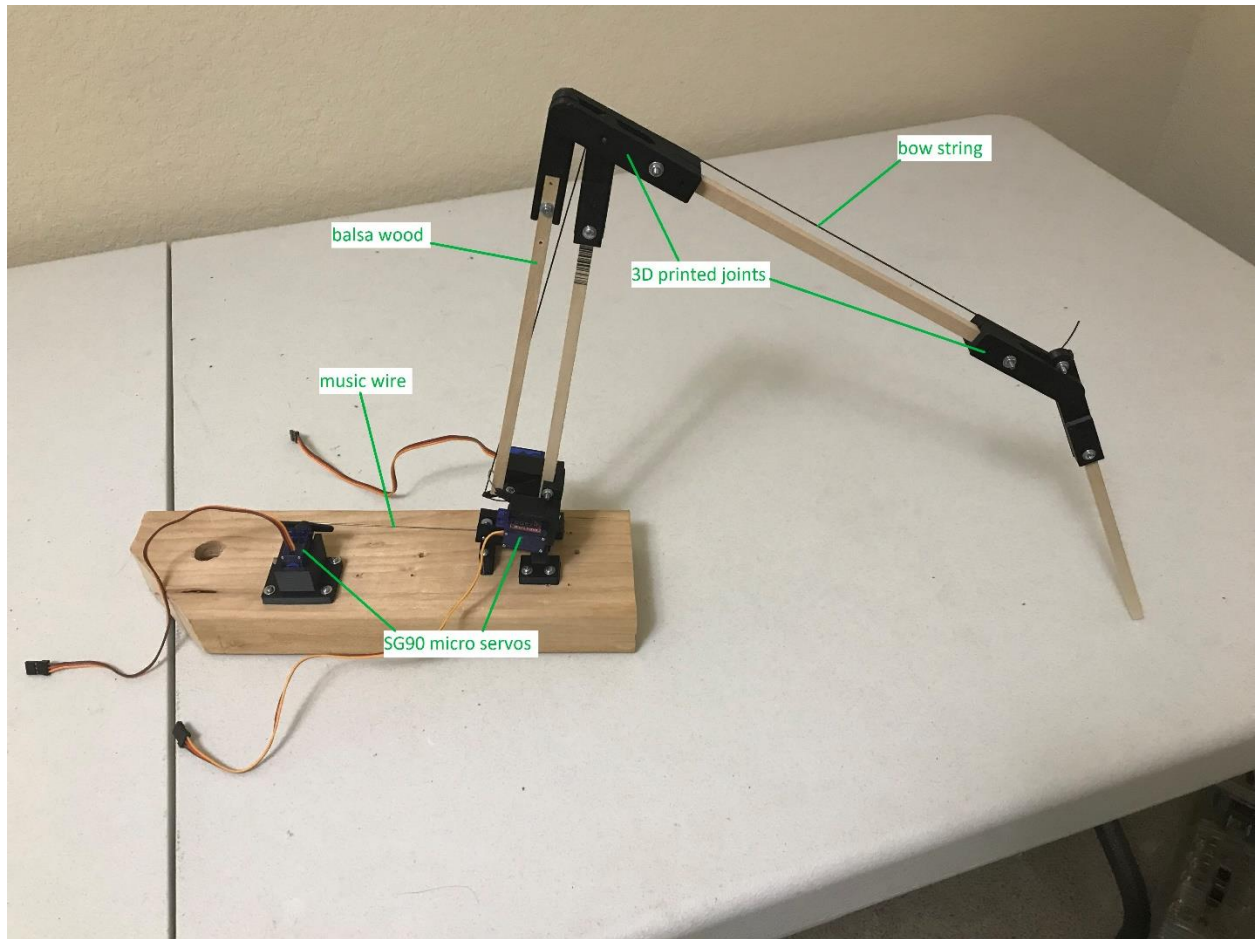
Leg: next prototype
