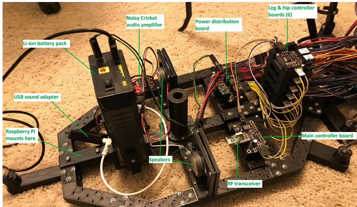
Spider electronics layout
