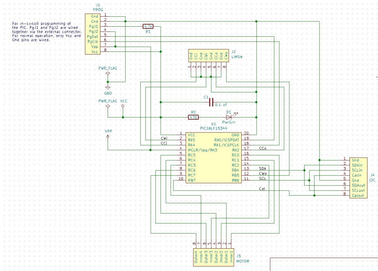
Leg control circuit
