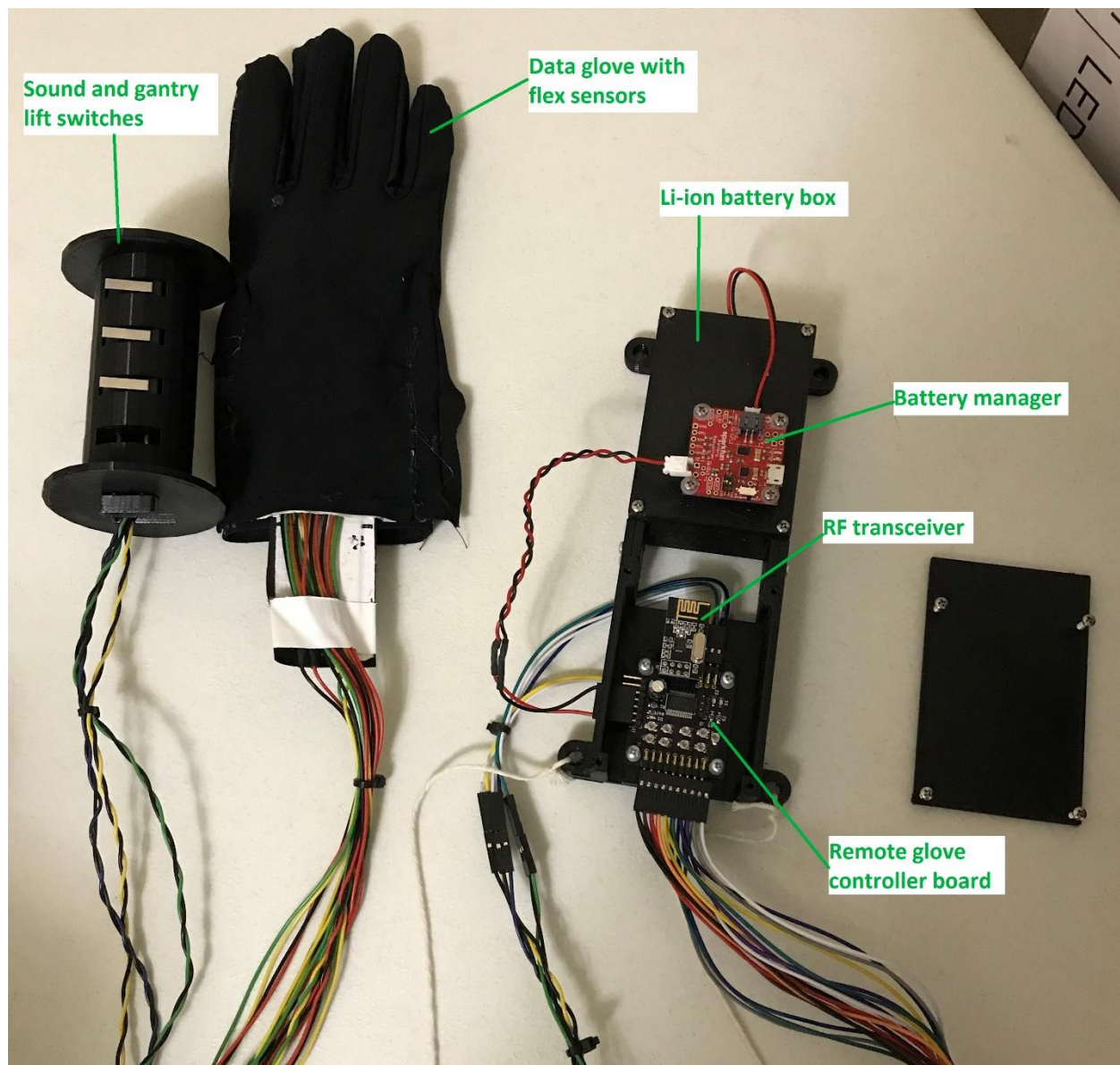
Glove electronics
