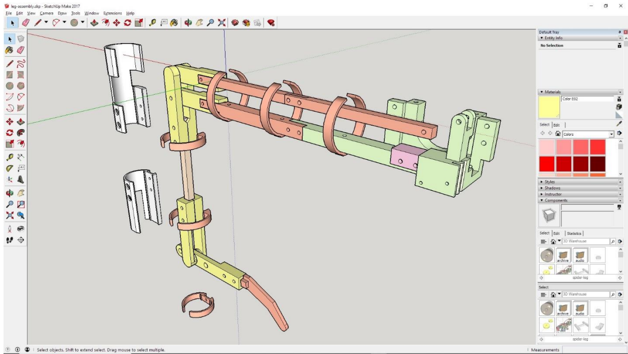
Spider leg assembly
